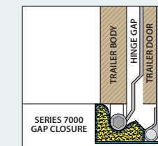
Detail of Patented Gap Closure Device In Operation
