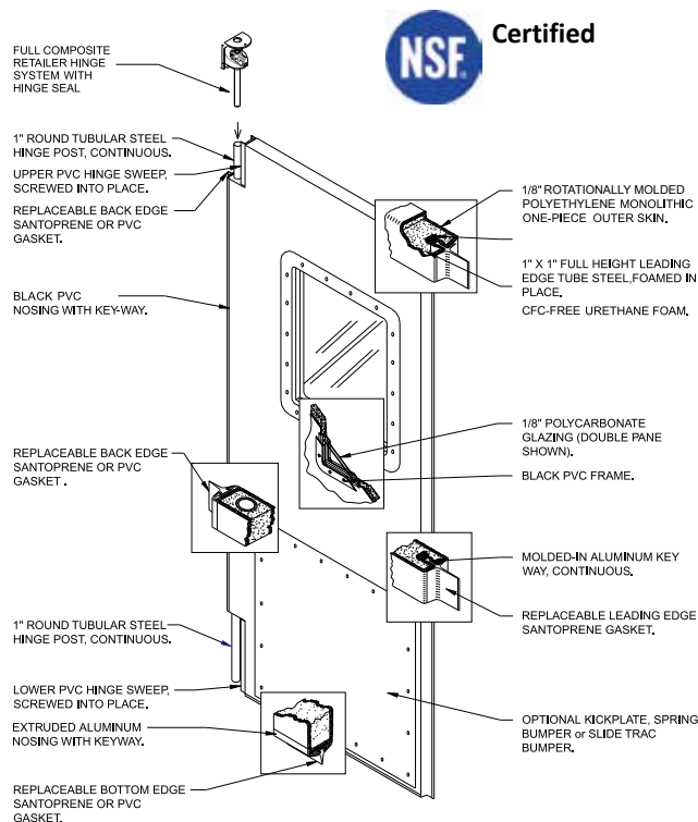
Durulite Retailer Shown with Optional Impact Plates
